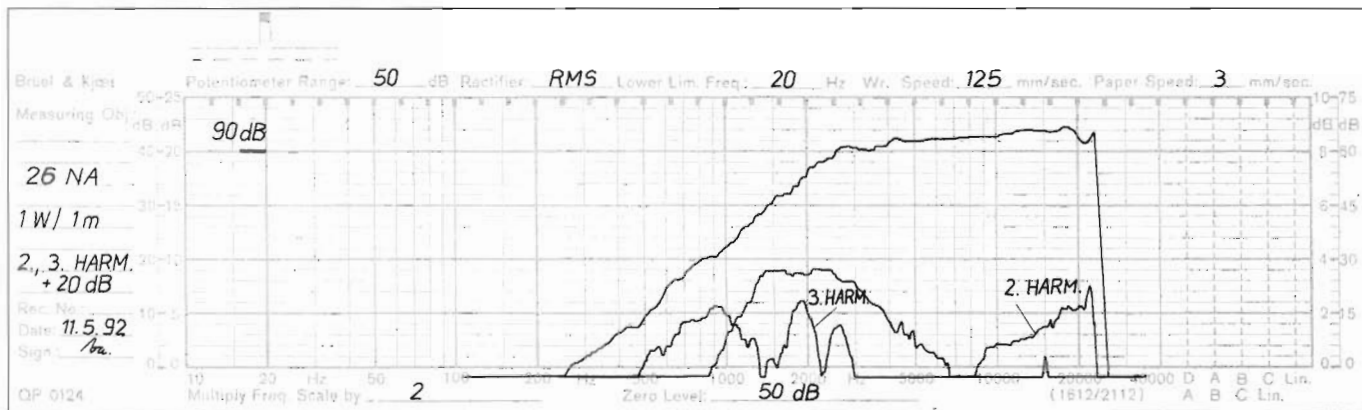
Frequency Response/Distortion
