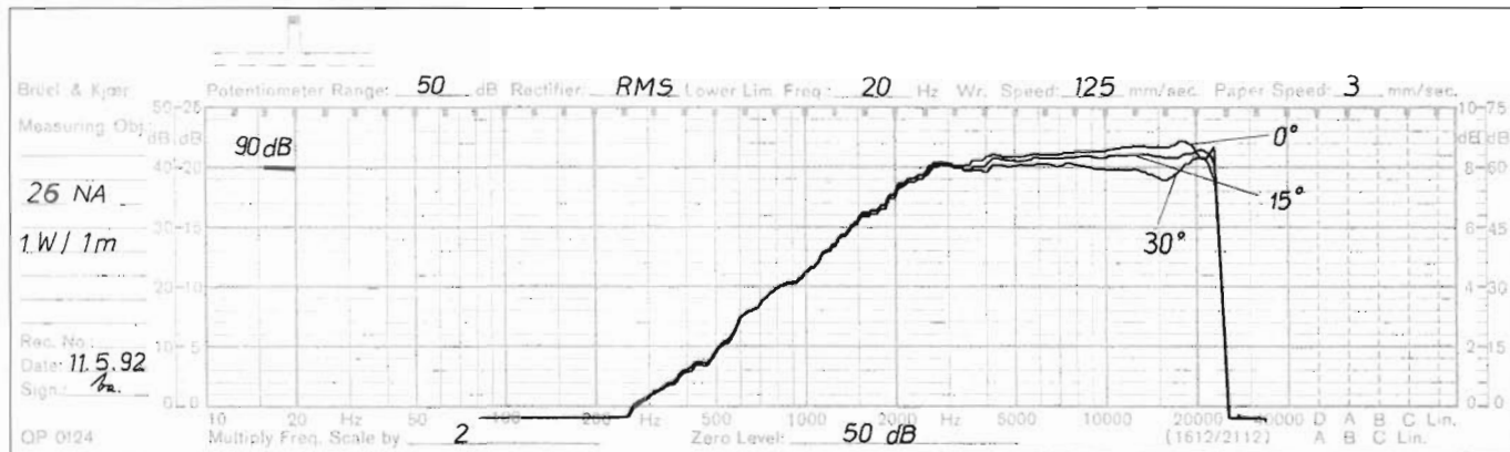
Frequency Response
